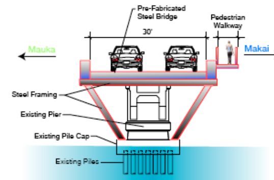
Bridge Cross Section
